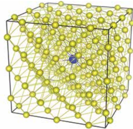
Supercell model used in the atomistic simulations to determine the degree of strengthening in Al (yellow atoms) using substitutional elements (blue atom).
